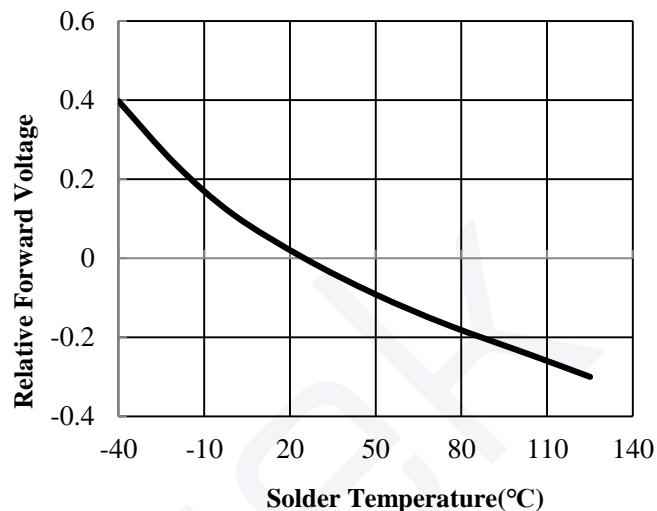
Forward Voltage vs. Solder Temperature
