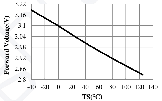
Forward Voltage vs. Solider Temperature
