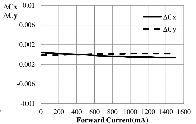
Chromaticity Coordinate Shift vs. Forward Current
