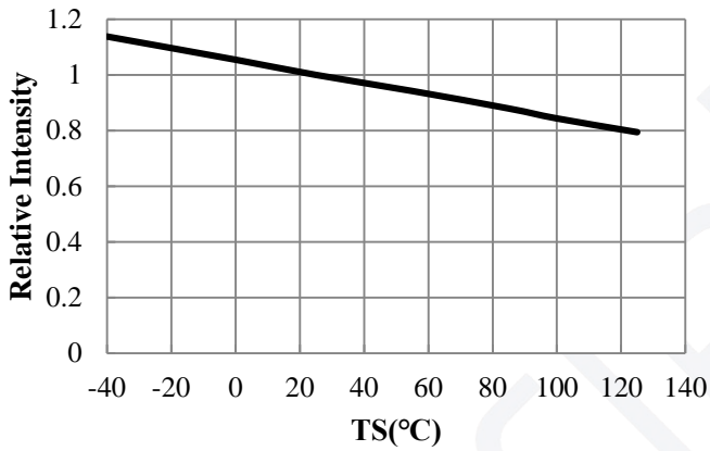
Relative Luminous Flux vs. Solider Temperature
