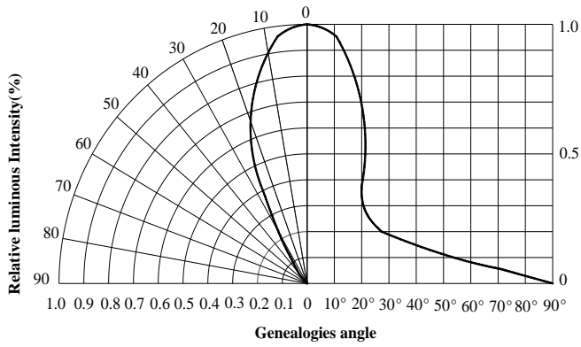
Radiation Characteristics
