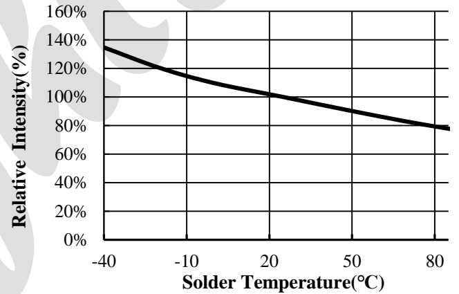
Relative Luminous Intensity vs. Temperature
