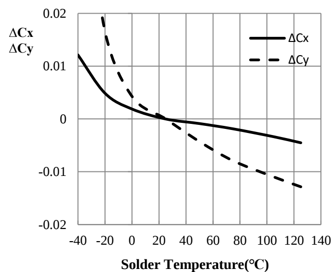
Chromaticity Coordinate vs. Solder Temperature
